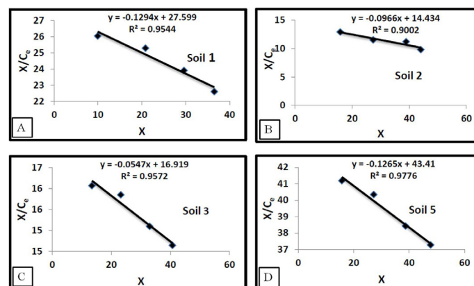
Figure 1: Thermodynamic equilibrium constant ( K_t ) for the studied soil samples in CaCl 2 saline solution at a temperature of 298K, A) Al-Shatra, B) Al-Dawaea, C) Al-Naser, and D) Al-Alkalaa soil samples.
