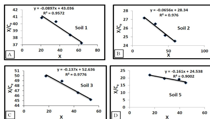
Figure 3: Thermodynamic equilibrium constant ( K_t ) for the studied soil samples in CaCl 2 saline solution at a temperature of 318K, A) Al-Shatra, B) Al-Dawaea, C) Al-Naser, and D) Al-Alkalaa soil samples.
