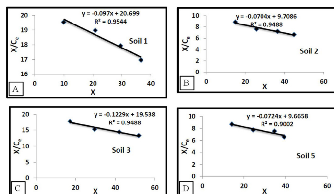
Figure 2: Thermodynamic equilibrium constant ( K_t ) for the studied soil samples in NaCl solution at a temperature of 298K, A) Al-Shatra, B) Al-Dawaea, C) Al-Naser, and D) Al-Alkalaa soil samples.
