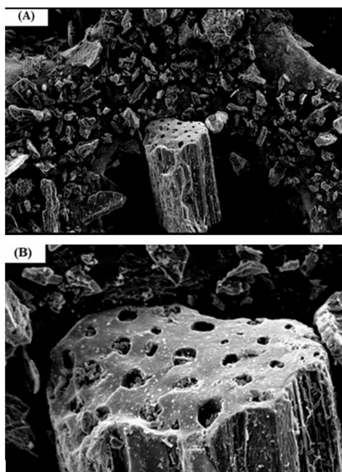
Figure 6: A and B: SEM images of the char from co-pyrolysis of SCB: WRT with KOH catalyst.
