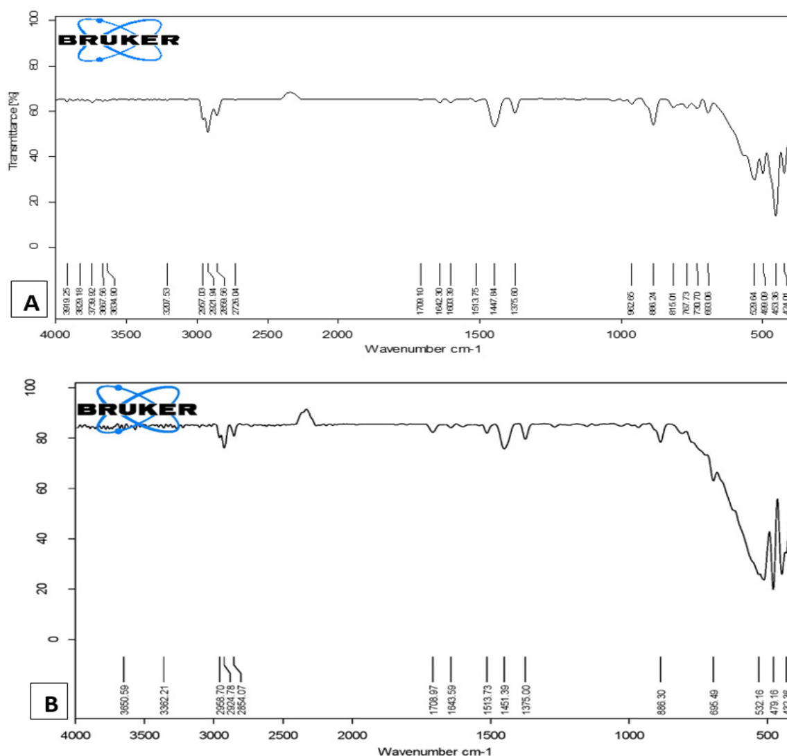
Figure 7: FTIR analysis of (A) SCB and (B) RH: WRT mixture with KOH as catalyst.
