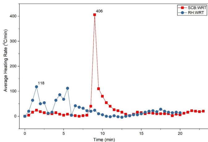
Figure 3: Average heating rates of co-pyrolysis of RH:WRT and SCB:WRT.
