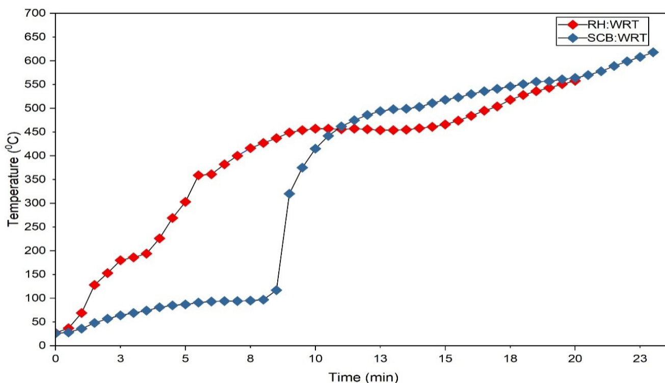
Figure 1: Temperature profile of co-pyrolysis of RH: WRT and SCB: WRT.
