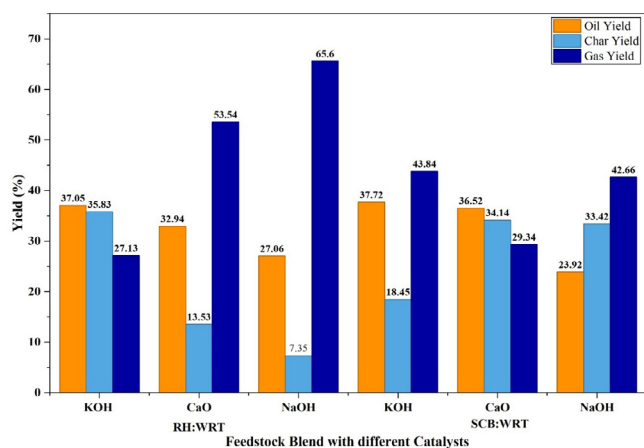
Figure 4: Effect of catalysts on feedstock blend.
