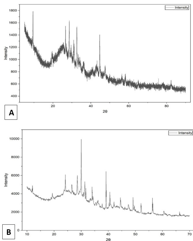
Figure 5: XRD spectrum of char from co-pyrolysis of (A) SCB: (B) RH:WRT with KOH catalyst.
