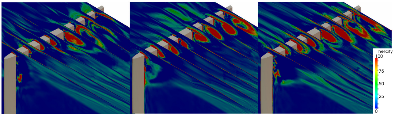
Figure 5: Tip leakage vortices evolution by the helicity contours.
