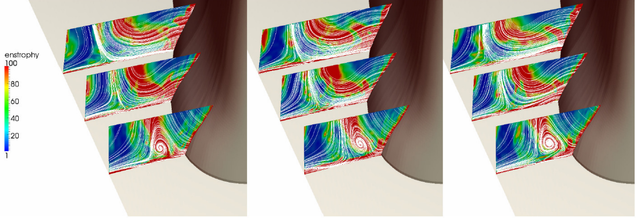
Figure 6: Horse-shoe vortex visualization by enstrophy contours and streamlines.
