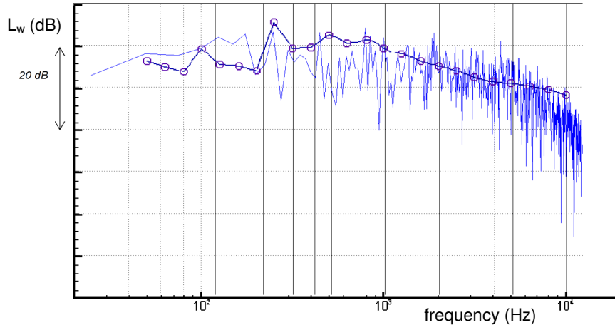
Figure 8 - Comparison of sound power level spectra at design condition (line-symbol: experiments; line: computation)
