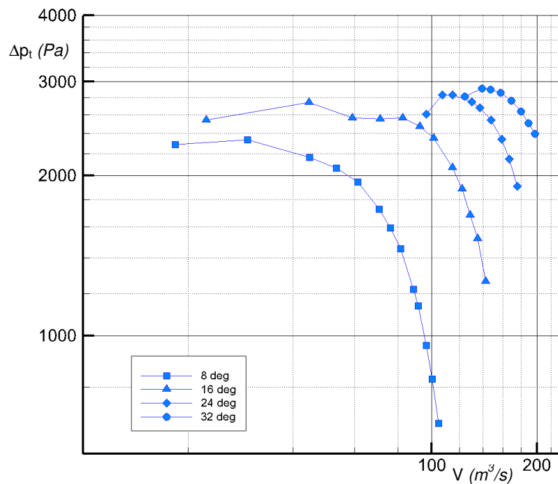
Figure 2: Total pressure-volume operating margin 224JFM
